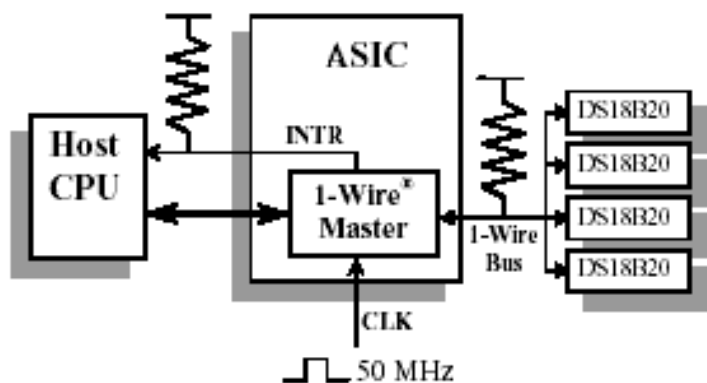
Figure 1. Example Circuit
